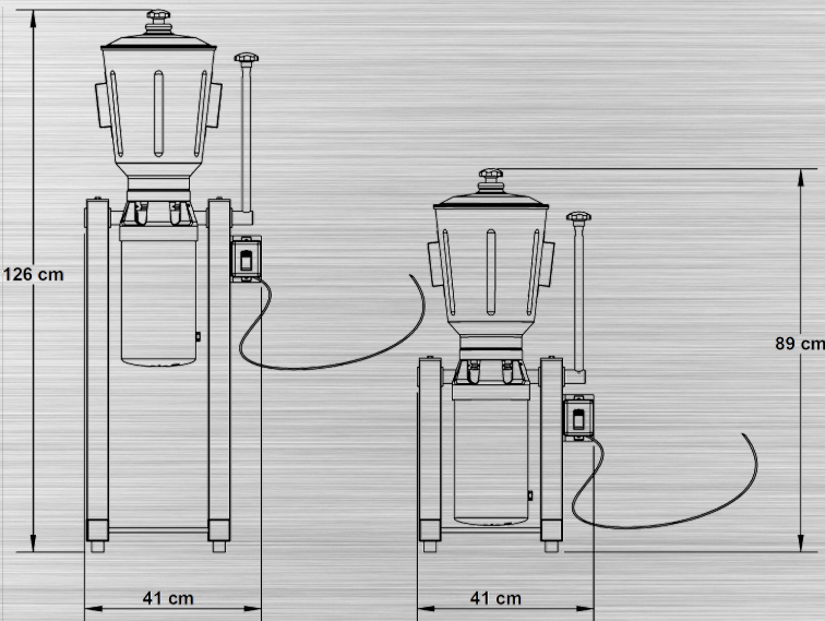
Vista frontal
